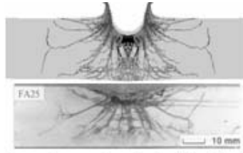
Ceramic armor impact: simulation (top)
