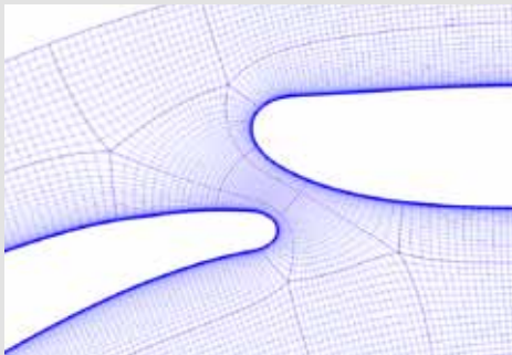
Quality and shape remain consistent with mesh refinement
