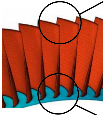
The ATM method adjusts to maintain mesh quality as blade shape changes along the span
