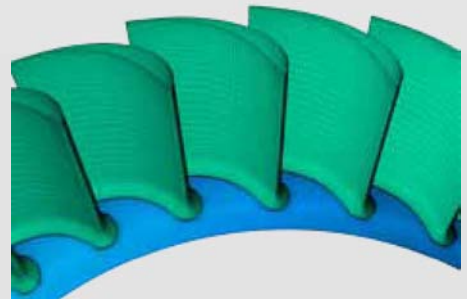
High-quality meshes for blades with fillets
