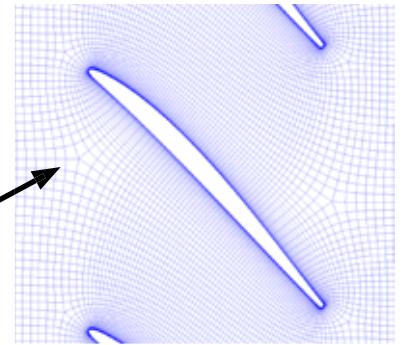
The ATM method adjusts to maintain mesh quality as blade shape changes along the span
