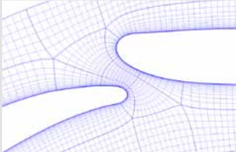
Quality and shape remain consistent with mesh refinement
